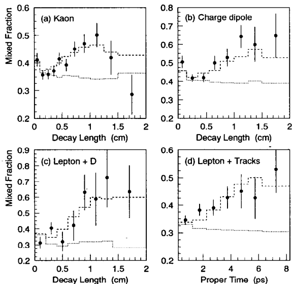
Figure 4. Distributions of the fraction of decays tagged as mixed as a function of decay length or proper time for data (points) and best fit MC (dashed histograms) for the various analyses: (a) charged kaon, (b) charge dipole, (c) lepton + D , and (d) lepton + tracks. The dotted histograms correspond to MC distributions with no B_d^0 - \bar{B}_d^0 mixing.
