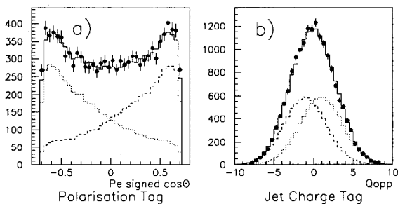
Figure 3. Distributions of (a) polarization-signed \cos\theta_T and (b) opposite hemisphere jet charge for data (points) and MC (solid line). The MC b and \bar{b} components are shown with dotted and dashed lines respectively.
