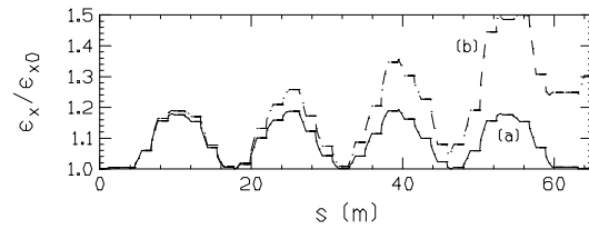
Figure 2. Fractional CSR emittance growth in arc for a constant 25\text{-}\mu\text{m} bunch (a) and a compressing bunch of 25\text{-}\mu\text{m} (b). The charge is 2\text{ nC} and input emittance is \gamma\varepsilon_0 = 1\text{ }\mu\text{m} .
