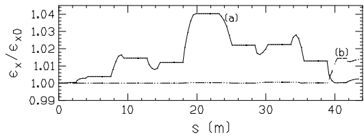
Figure 4. Fractional CSR emittance growth in wiggler of Fig. 3 for a constant 1-mm bunch length (a) and for a compressing bunch of 9-0.6 mm (b). The charge is 6 nC and input emittance is \gamma\epsilon_{x0} = 8 \mu\text{m} .
