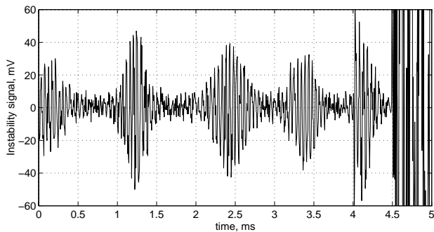
Figure 3. Instability signal after the detector
