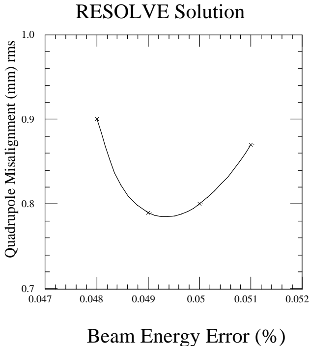
Figure 3. A plot of the solution for different beam energy error values for a case with simulated error of 0.05%.
