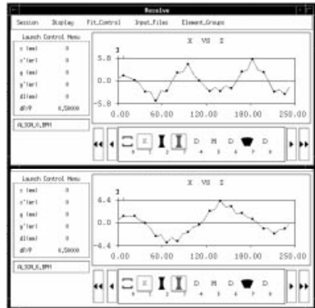
Figure 2. Typical trajectories used in our example.
