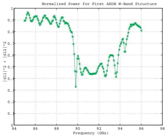
Fig9: The sum of the squares of the reflection coefficient and the transmission coefficient.
