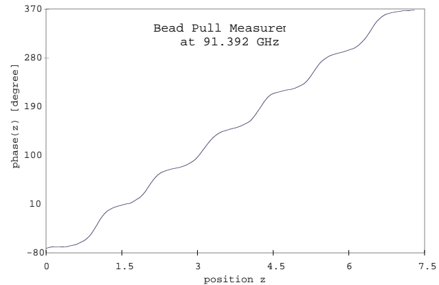
Fig11: The measured phase advance (degrees) of the accelerating field along the structure.
