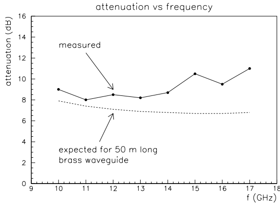
Figure 6: Measured attenuation of TE_{10} mode.
