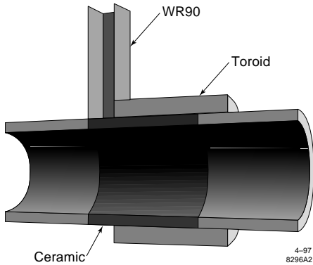
Figure 4: Model for the numerical calculation of beam-waveguide coupling using MAFIA [4].
