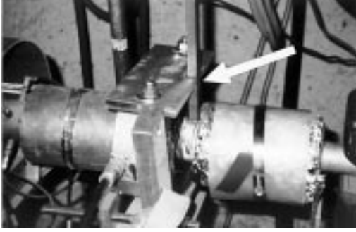
Figure 3: Waveguide pickup (arrow), toroid (left from waveguide), ceramic gap (below waveguide) and bellows (left and right), in the SLC South Final-Focus beam pipe.
