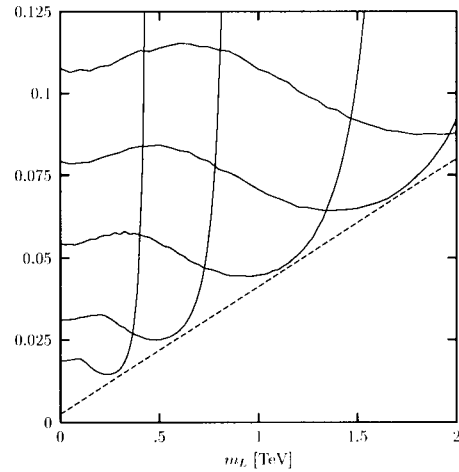
Figure 10: Smallest observable scalar bilepton coupling as a function of the bilepton mass at the level one standard deviation in e\gamma processes. The assumed e^+e^- center of mass energies are 0.5, 1, 2, and 3 TeV, from left to right. (From Ref. [26].)
