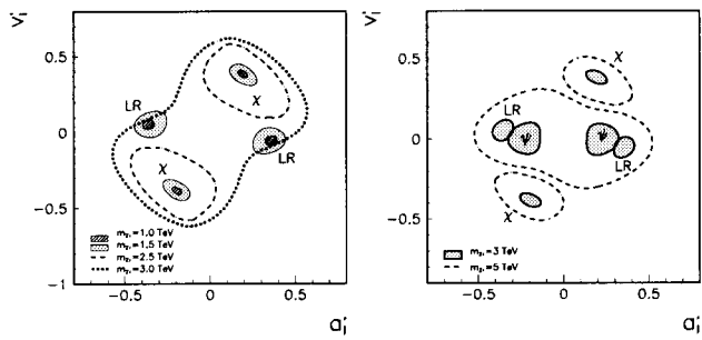
Figure 4: 95% C.L. contours for a'_\ell and v'_\ell . A Z' is assumed in the \chi , \psi , or LR model for different Z' masses. The left and right figures are for \sqrt{s} = 500 GeV, L = 50 fb^{-1} and \sqrt{s} = 1.5 TeV, L = 100 fb^{-1} . (From Ref. [19].)
