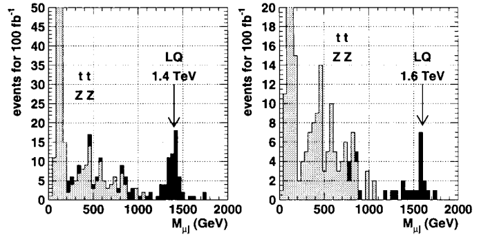
Figure 7: Leptoquark signal and background mass distribution for second generation leptoquarks for the CMS detector. (From Ref. [28].)
