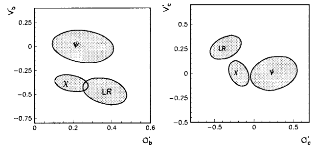
Figure 5: Model discrimination for M_{Z'} = 1 TeV at \sqrt{s} = 0.5 TeV with L=50 fb^{-1} for e^+e^- \rightarrow bb (left) and e^+e^- \rightarrow cc (right). 60% (40%) tagging efficiencies and 1% (1.5%) systematic errors were used for b ( c ). (From Ref. [19].)
