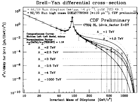
Figure 19: Comparison between CDF Drell-Yan cross-section measurement and the theoretical predictions for various values of the scale \Lambda_{LL}(qqee) (for \eta = -1 ) for the dielectron channel. From ref. [50]
