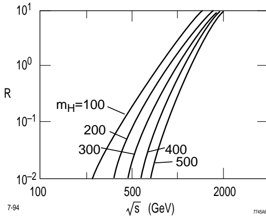
FIGURE 7. Production cross sections, by an NLC/TLC e^-e^- collider, of doubly charged H^{--} bosons in the mass range from 100 to 500 \text{GeV}/c^2 , in units of R.
