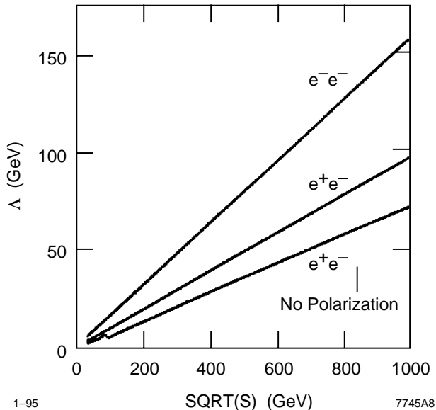
FIGURE 16. The 95% CL limits that can be obtained for the compositeness scale \Lambda_{LL} as a function of the e^-e^- or e^+e^- center-of-mass energy. The luminosity is given by \mathcal{L} = 680 \text{ pb}^{-1} \times s/M_Z^2 . The polarization of the electron beam(s) is indicated in the figure.
