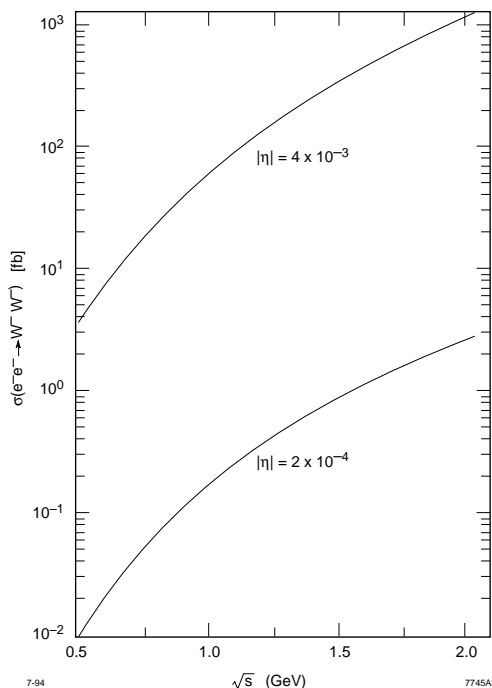
FIGURE 19. Energy dependence of the cross-section for the process e^-e^- \rightarrow W_L^-W_L^- in the energy range of an NLC-type machine of a typical luminosity 10\text{--}100\text{ fb}^{-1} , for the range of neutrino mass matrix choices discussed in Ref. [18].
