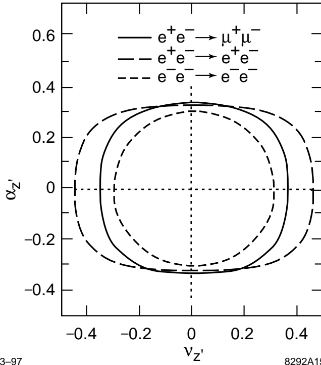
FIGURE 17. Contours of observability of Z' coupling to a Z' of 2 TeV mass.
