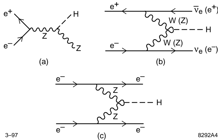
FIGURE 1. (a) ‘‘Higgs radiation’’: e^+e^- annihilation into a virtual Z boson followed by ‘‘Higgsstrahlung’’; (b) WW fusion and ZZ fusion in e^+e^- collisions; (c) central production of Higgs boson in e^-e^- collisions. H^0 mass can be reconstructed if outgoing electron momenta are measured.
