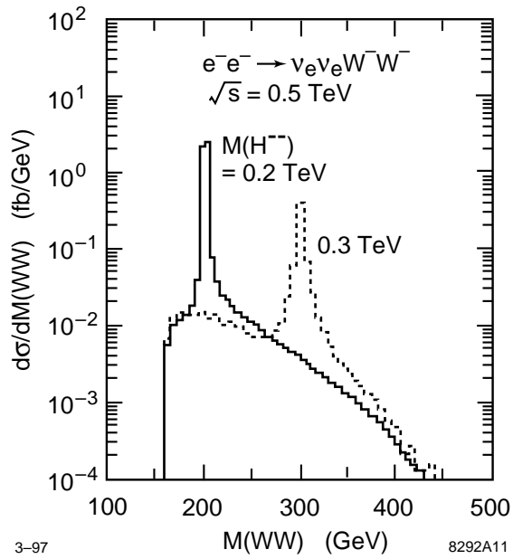
FIGURE 13. Distribution in the W^- W^- invariant mass for e^- e^- \rightarrow \nu_e \nu_e W^- W^- , including the contribution of a doubly-charged Higgs boson of mass M(H^{--}) = 0.2 or 0.3 TeV.
