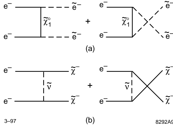
FIGURE 8. (a) \tilde{e} pair production from e^-e^- collisions by \tilde{\chi}_1^0 exchange. (b) Like-sign \tilde{\chi}^- pair production by \tilde{\nu} exchange.
