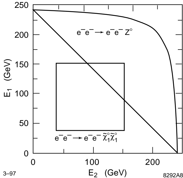
FIGURE 10. Permitted energy range for the two electrons observed in the two reactions mentioned in the figure. For \tilde{e} decay, we assumed m(\tilde{e}) = 200 GeV, m_{\tilde{\chi}^0} = 100 GeV. The diagonal cut eliminates the background while losing little signal.
