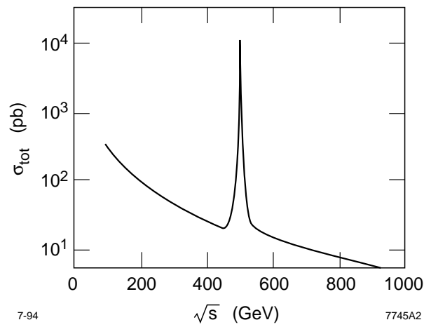
FIGURE 18. Production cross-section, as a function of energy, of dilepton gauge bosons in e^-e^- collisions. The 500 GeV mass and narrow width were assumed for illustration purposes.
