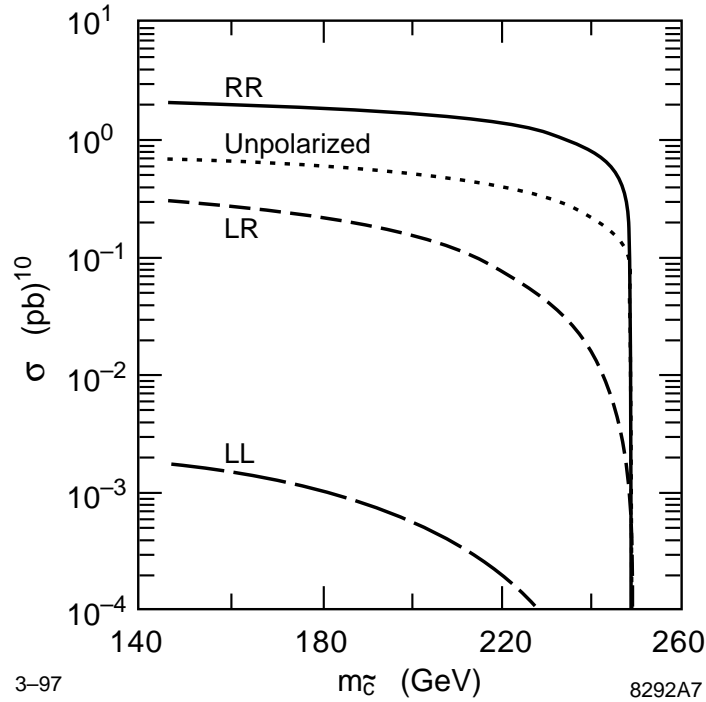
FIGURE 9. Cross-section for \tilde{e}^- pair production from e^-e^- collisions as a function of \tilde{e} mass, for an e^-e^- collider of \sqrt{s} = 500 GeV, with the incident electron helicities as indicated. For SUSY parameters see Ref. [7].
