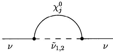
FIG. 1. One-loop contribution to the neutrino mass due to sneutrino mass splitting.
