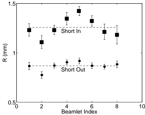
Figure 6: Beamlet centroid position from center beamlet
