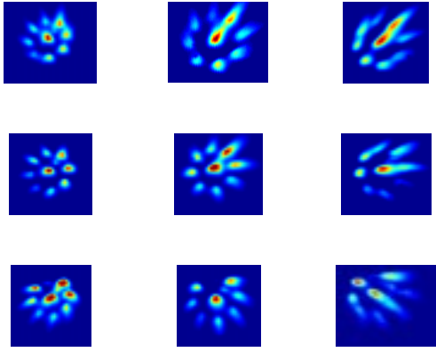
Figure 5: Beamlets profile with the rf gun unsymmetrized
