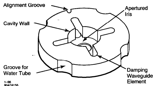
Figure 4: Schematic DDS structure; from Ref. [1].
