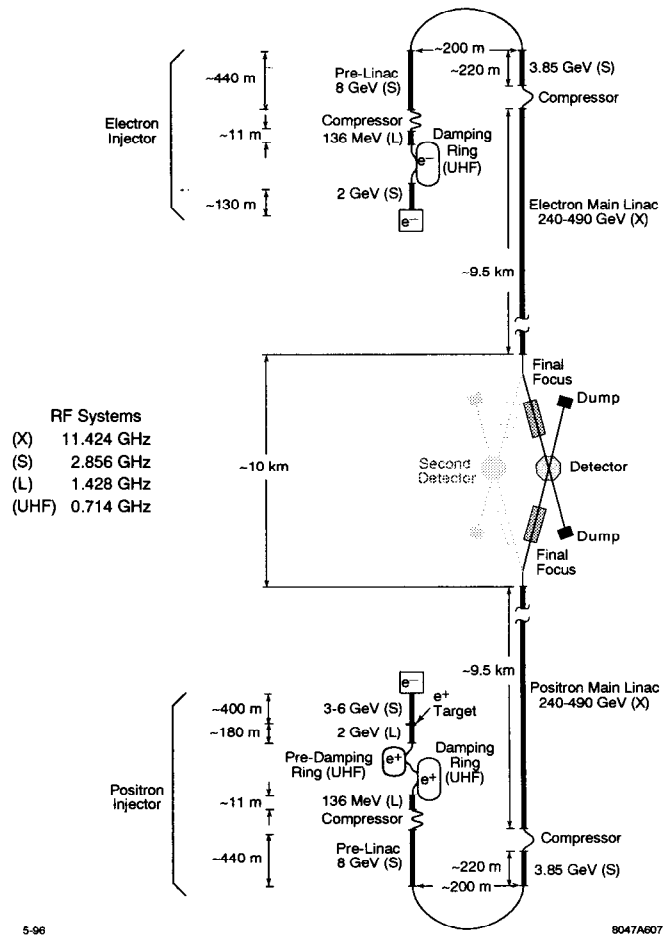
Figure 2: Schematic of the NLC; from Ref. [1].
