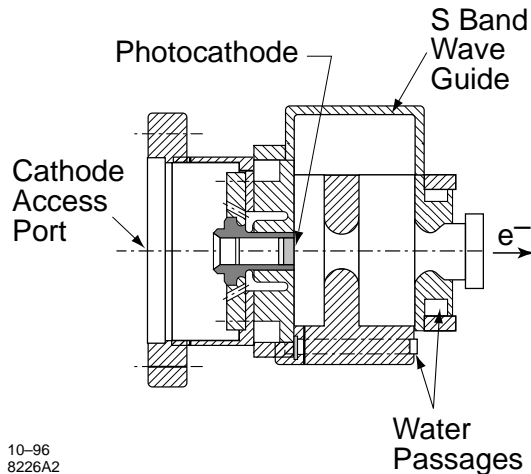
Figure 2: Cross section of rf gun.
