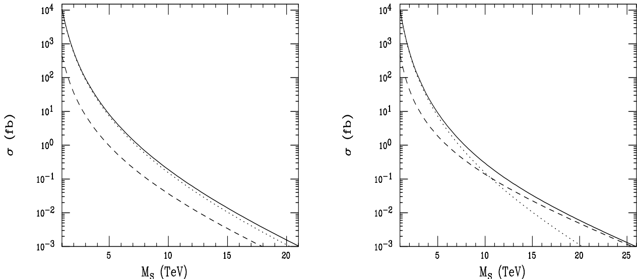
Figure 4: Same as Fig.2 but now at the 200 TeV PIPETRON collider.
