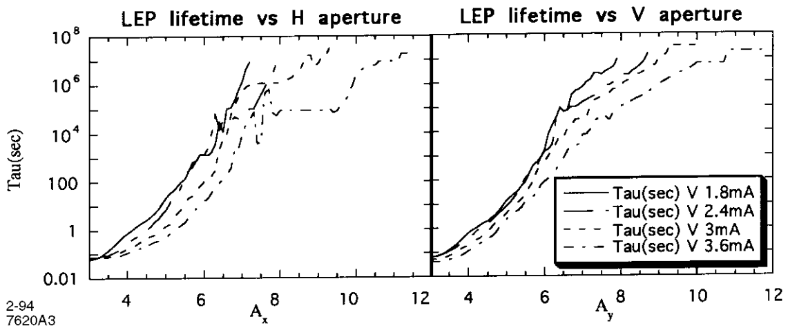
Figure 3. The lifetime as a function of horizontal and vertical apertures for different beam currents.
