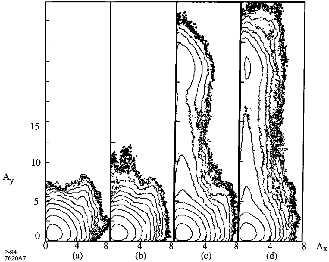
Figure 7. Distributions with high second order vertical chromaticity. (a) Q_y'' = -1 \times 10^3 ; (b) Q_y'' = -4 \times 10^3 ; (c) Q_y'' = -8 \times 10^3 ; (d) Q_y'' = -1.5 \times 10^4 . These chromaticities are for the one-quarter LEP model. Other parameters are the those in Table I and Table II, Group 2 .
