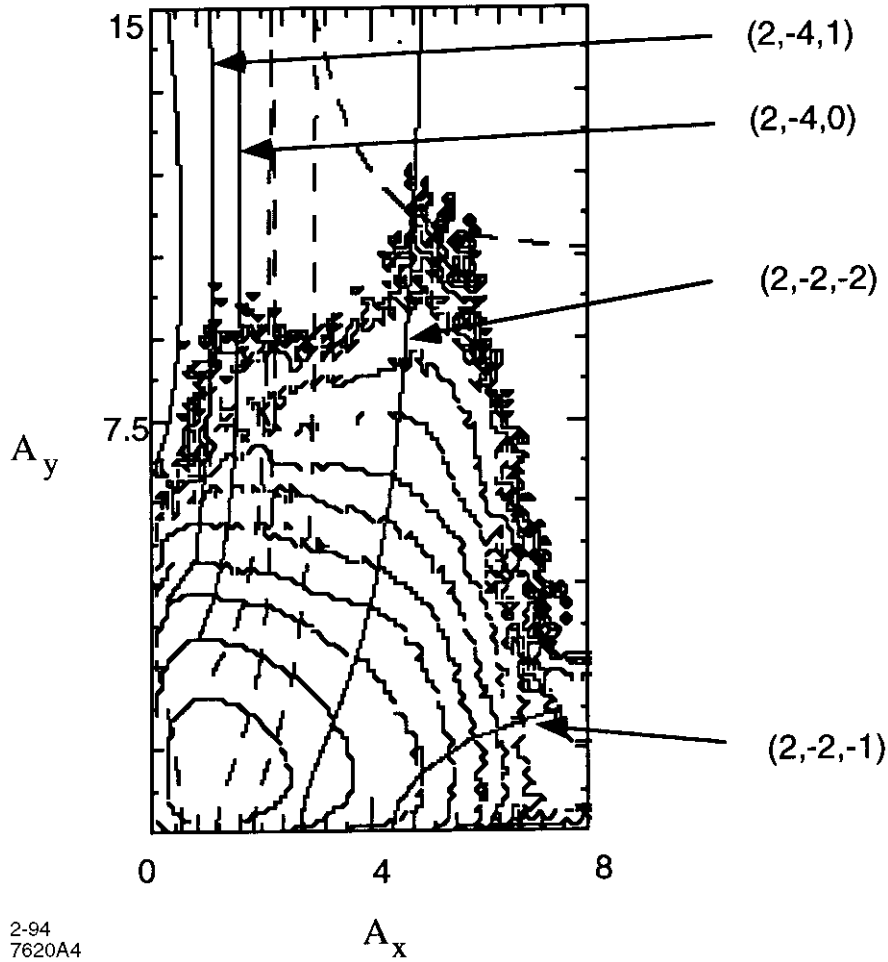
Figure 4. The location of resonances in amplitude space superimposed on the beam distribution from Figure 1d. The resonances are of a form pQ_x + rQ_y + mQ_s = n , and the lines are labeled as (p, r, m) .
