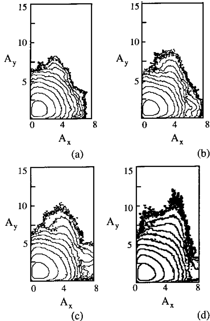
Figure 1. Logarithmic contours of particle number. (a) I_b = 1.8\text{mA} ( \xi_x = 0.034 , \xi_y = 0.021 ); (b) I_b = 2.4\text{mA} ( \xi_x = 0.046 , \xi_y = 0.027 ); (c) I_b = 3.0\text{mA} , ( \xi_x = 0.057 , \xi_y = 0.034 ); (d) I_b = 3.6\text{mA} , ( \xi_x = 0.069 , \xi_y = 0.041 ).
