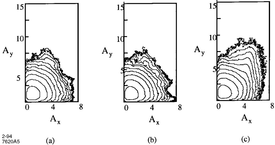
Figure 5. Distributions with: (a) no amplitude dependent tunes due to lattice nonlinearities (identical to Figure 1a); (b) lattice nonlinearities in Table II, Group 1 ; (c) lattice nonlinearities, parameters in Table II, Group 2 .
