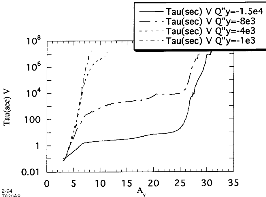
Figure 8. Lifetime versus vertical aperture with different Q_y'' .
