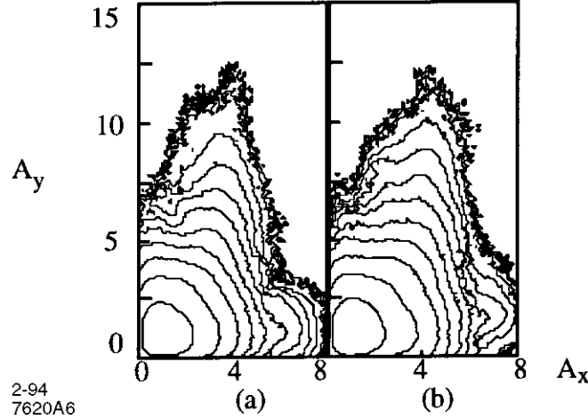
Figure 6. Tail distributions with increased \xi and lattice nonlinearities. Most parameters are the same as Table I together with Table II, Group 2 , but the beam current and sizes are changed to obtain higher \xi 's. (a) uses the parameters in Table III, Group A ; (b) uses the parameters in Table III, Group B .
