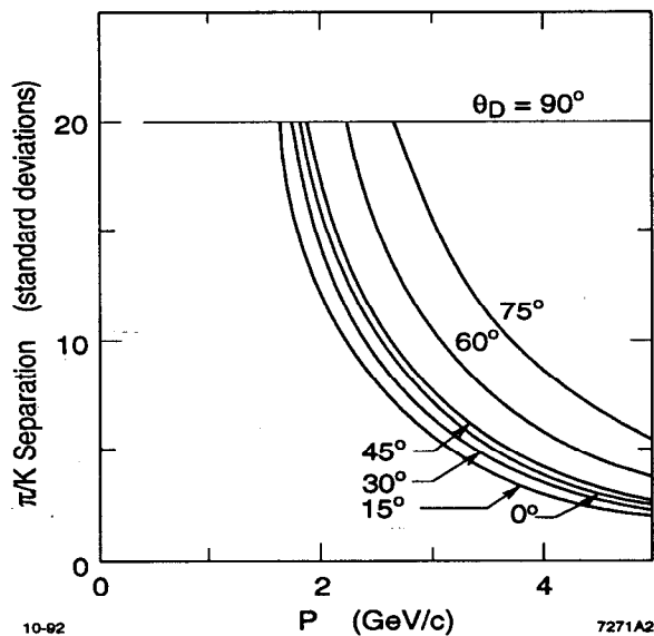
Figure 9. The predicted \pi/K separation as a function of momentum in a DIRC counter with a detector resolution of 6.8 mr. The lines show the dependence for a variety of track dip angles \theta_D .
