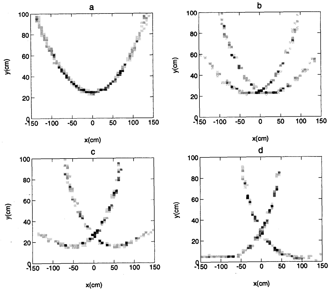
Figure 8. Loci of Cherenkov images from a \beta = 1 track on a cylindrical detection surface 100 cm from the radiator end. The track is at a dip angle ( \theta_D ) of 30^\circ and images are shown for four different azimuthal angles (a) 0^\circ , (b) 10^\circ , (c) 20^\circ , and (d) 30^\circ .
