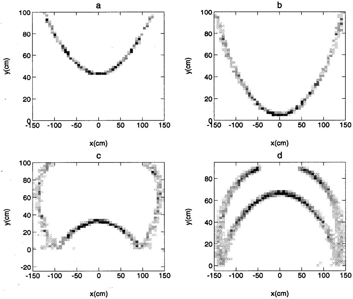
Figure 7. Loci of Cherenkov images from a \beta = 1 track on a cylindrical detection surface 100 cm from the radiator end. The track enters the radiator perpendicularly in azimuth. Dip angles of (a) 20^\circ , (b) 40^\circ , (c) 60^\circ , and (d) 80^\circ are shown.
