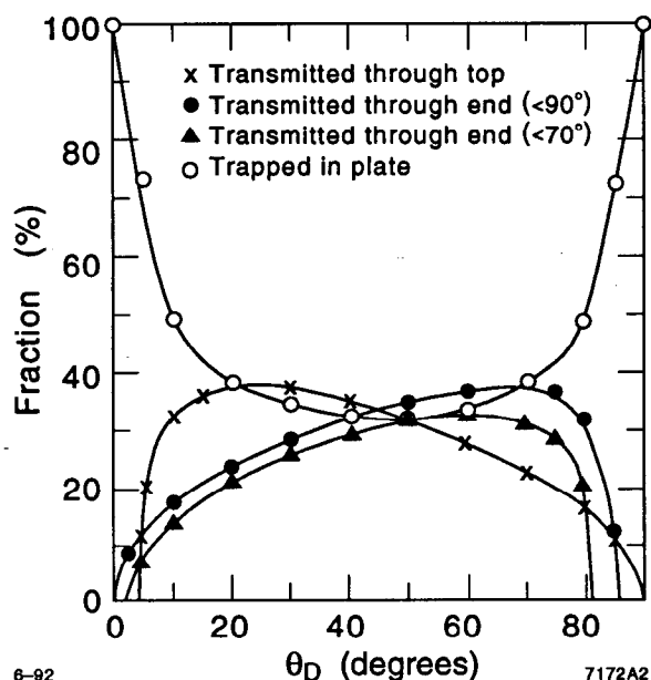
Figure 3. An accounting of the fate of the photons in a quartz radiator ( \langle n_1 \rangle = 1.474 ) as a function of the dip angle for a \beta=1 track. The standoff region is air ( n_2 = 1.0 ). The open circles indicate that a large fraction of the light is trapped, especially near zero and ninety degrees.
