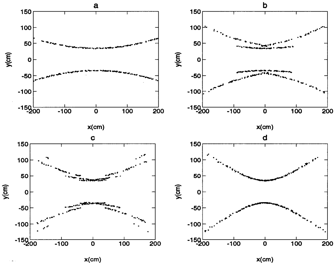
Figure 2. Loci of images for a \beta = 1 track at a dip angle of 30^\circ for radiator widths of (a) t_x=1000 cm (b) t_x=100 cm (c) t_x=20 cm (d) t_x=5 cm. The track azimuthal angle ( dx/dy ) is zero. The radiator is quartz ( \langle n_1 \rangle = 1.474 ) and the detector standoff region is air ( n_2 = 1.0 ). The distance of the detector from the radiator is 100 cm. The track enters at t_x/2 and at 100 cm from the end of the 1cm thick radiator.
