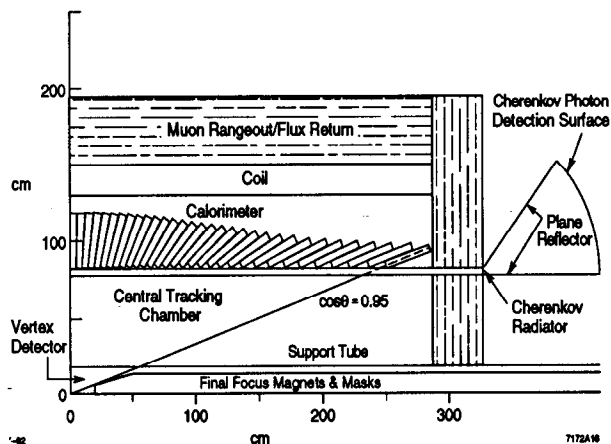
Figure 6. Schematic view of one quadrant of a B Factory detector incorporating a DIRC
