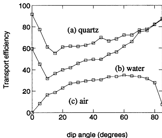
Figure 4. The fraction of Cherenkov photons from a \beta=1 track transmitted to the detector as a function of dip angle for various refractive indices in the standoff region (a) quartz ( n_2=1.474 ), (b) water ( n_2=1.34 ) and (c) air ( n_2=1.0 ). The radiator is quartz ( \langle n_1 \rangle=1.474 ). Note the improvement in efficiency for small dip angles as n_2 approaches n_1 , due to improved collection of light reflected from the non-readout end of the radiator.
