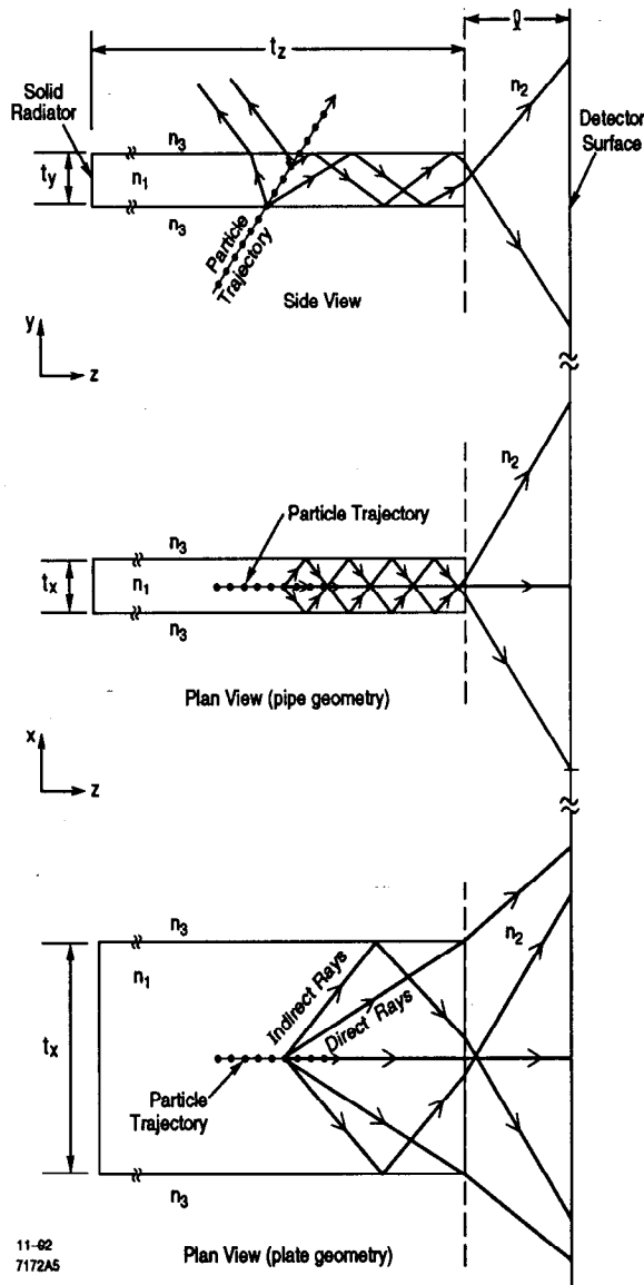
Figure 1. Schematic of a radiator bar of the DIRC counter for two different radiator widths (pipe and plate) described in the text; the particle trajectory is shown as a line connected by dots; representative trajectories of Cherenkov photons are shown by lines with arrows.
