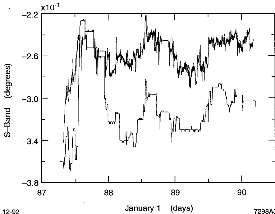
Fig. 3: Data from a beam phase monitor at the start of the linac(top trace). Phase adjustments made by operators at the start of the linac(bottom trace). Beam stability was poor from the start of the data to mid-morning of day 88. This produced the poor correlation between the operator phase adjustments and the beam phase monitor data seen for this period.
