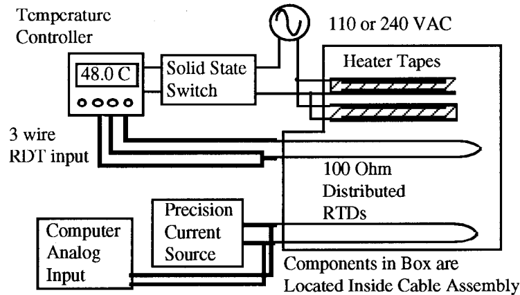
Fig. 5: Block diagram of equipment used for temperature control and readback of temperature stabilized cables. Two distributed RTDs run the length of the coaxial cable(s). One RTD is connected to a temperature controller which measures the average temperature of the cable, and cycles power to the heater tapes to maintain the desired cable temperature. The voltage drop across the second RTD is measured by an analog to digital module.
