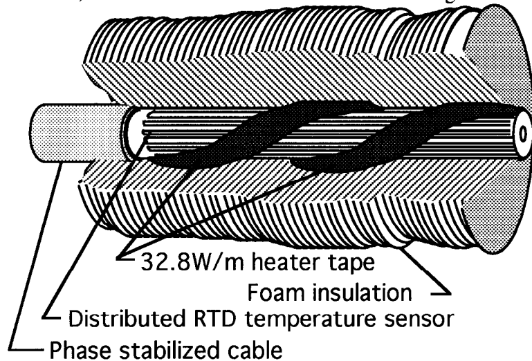
Fig. 4: Cut away of a section of temperature stabilized cable. The distributed RTD (resistance temperature detector) is connected to a standard temperature controller which measures the average temperature of the cable and cycles power to the heater tapes to keep this temperature constant.
