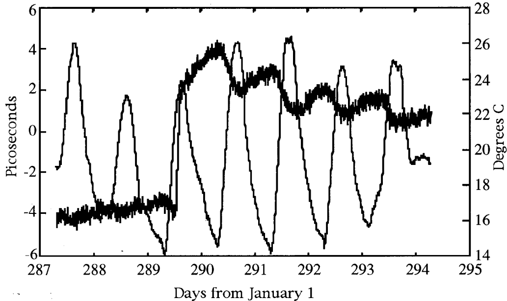
Fig. 5. Plot showing the propagation delay change in picoseconds of a temperature stabilized cable (thick trace), and the outside air temperature °C (thin trace). Results of the cable propagation delay test indicate that for a 9.5 °C air temperature swing, the propagation delay change is about 0.4ps. The stabilization system was turned off at noon on day 289. The delay change for this cable with the same air temperature variation was again measured and found to be about 1.5 ps. The reason for the slope of the plot while the stabilization system is active is not known for certain. It is believed to be a hysteresis effect due to small temperature variations in sections of the cable. The slope after the system is turned off, is the hysteresis associated with the temperature cycling of entire cable.
