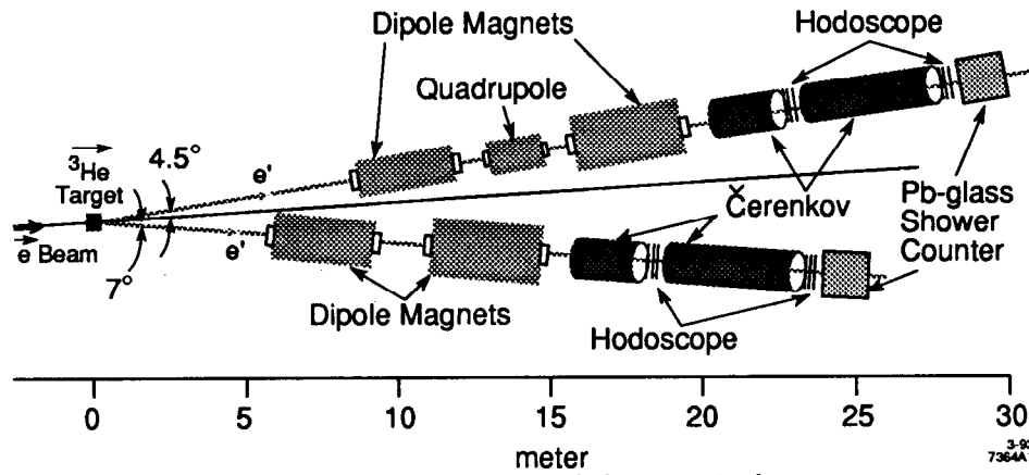
Figure 1. Experimental set up of the two single arm spectrometers.
