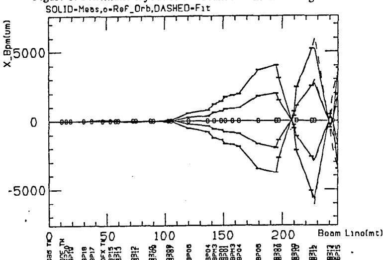
Figure 2. Beam orbit at different corrector values in the IP region as read from the BPMs with all the magnetic elements in the region [NBP06,SBP06] turned off.
