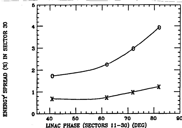
Figure 4 Energy spread at the end of the linac versus linac phase downstream of the compressor. The bunch charge is 3 \times 10^{10} compressed to \sigma_z = 0.083 mm in Sector 10. The (x) points used the nominal longitudinal wakefields in the Sectors 11-30. The (o) points used twice the nominal wakefields. The final beam energies are 25-35 GeV.
