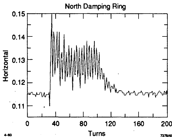
Figure 4. Raw data at the start of the cycle when less than 100 turns had been achieved.
