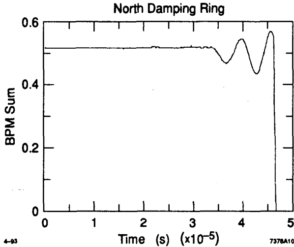
Figure 7. Data representing inverse bunch length just before extraction derived from a BPM sum signal.
