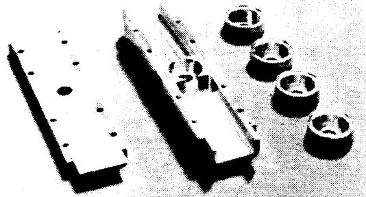
Figure 1. Input coupler and four cells of 30-cell structure.
