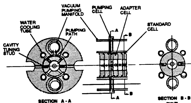
Figure 6. Design features of the 1.8 m structure.
