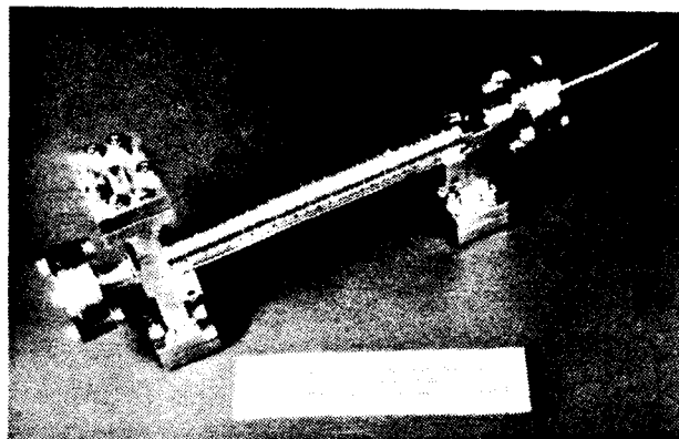
Figure 2. Completed 30-cell accelerator.
