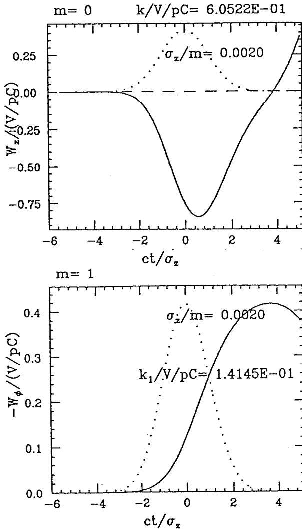
Figure 1: Wakefield Calculation.
