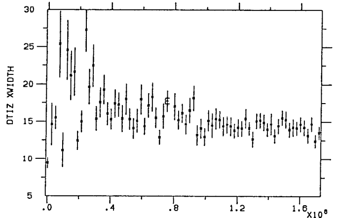
Figure 3: Injection oscillations of the bunch length.
