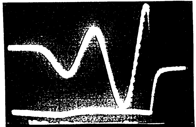
Figure 5: Pre-compression of the bunch length.
