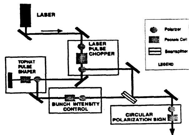
Figure 2. The Polarized Light Source for E142.
