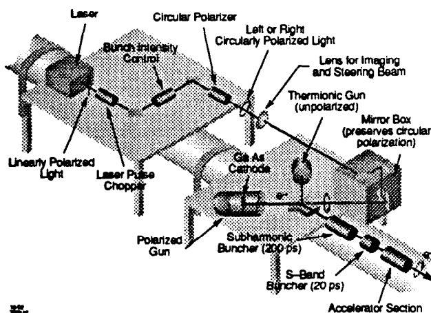
Figure 1. The Polarized Electron Source at SLAC.
