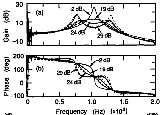
Figure 5: ALS measured versus fitted T_{A-B}^{cl}(s) for loop gains of -2, 19, 24 and 29dB.
