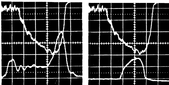
Figure 2. Current pulse (upper and inverted) directly out of the rf gun as compared in time, 0.5 \mu\text{s}/\text{div} , to (a) [left] the gun reflected rf power pulse (lower), and (b) [right] the current pulse (lower) after being scraped and compressed by the alpha magnet.
