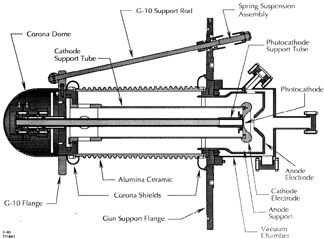
Figure 1. SLC photocathode diode gun. (See Ref. 3.)
