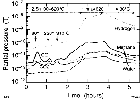
Figure 3. Partial pressures in the gun during cathode heat cleaning as measured with a VG Sensorlab RGA system.
