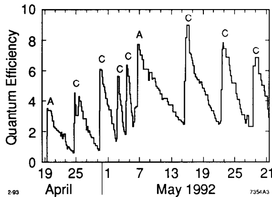
Figure 4. Quantum efficiency (750 nm and 120 kV) for first two activation cycles at the SLC injector. "A" indicates activation (heat cleaning/cesiation/fluoride), "C" indicates cesiation only. The initial QE had dropped to \sim 3.5\% by the time the plot began.
