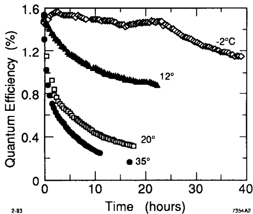
Figure 2. Temperature dependence of photocathode quantum efficiency lifetime.
