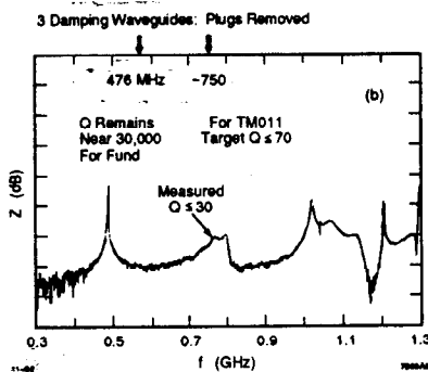
Figure 3. Damped low power RF cavity impedance.
