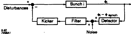
Figure 4. A schematic diagram of the bunch-by-bunch feedback scheme.
