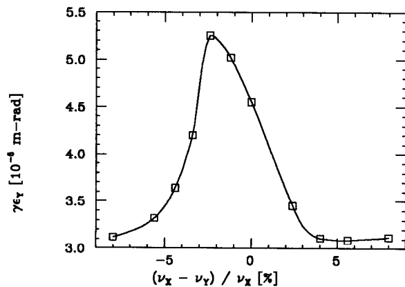
Fig. 5 Vertical emittance vs. difference between horizontal and vertical quadrupole focusing in the NLC pre-linac; the emittance is that of the 30th bunch and the partial pressure of CO is 10^{-7} Torr. Note the peak occurs when the horizontal focusing is weaker than the vertical.
