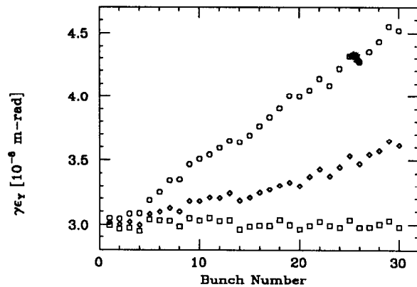
Fig. 4 Vertical emittance vs. bunch number in the NLC pre-linac at the beginning (squares), middle (diamonds), and end (circles); the linac has equal horizontal and vertical focusing of 90^\circ per cell and a CO partial pressure of 10^{-7} Torr.
