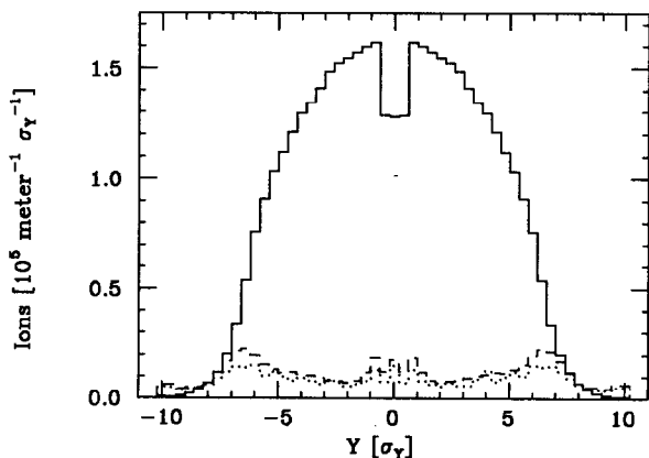
Fig. 3 Vertical projection of the ion density in the (old) NLC pre-linac after 1 bunch (solid), 2 bunches (dashed), 3 bunches (dotted) with a CO gas partial pressure of 10^{-7} Torr. Note that the ions are strongly over-focused by the beam.
