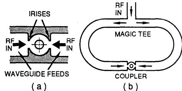
Fig. 1 Schematics of RF power input to coupler.
