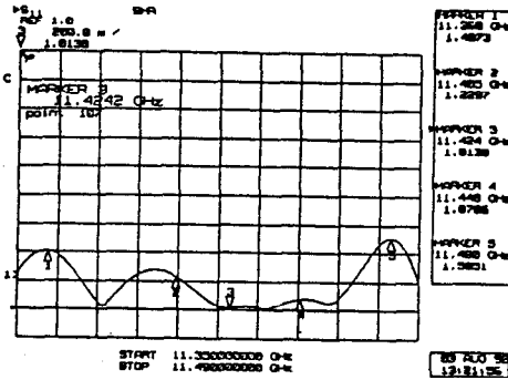
Fig. 6b Cold-test data of VSWR versus frequency.
