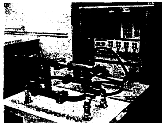
Fig. 3 Cold-test assembly.
