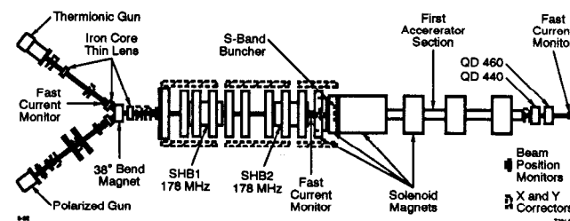
SCL injector beam line up to the fast current monitor at 40 MeV.
