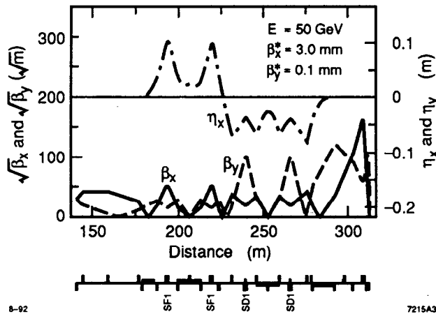
Fig. 3. Optics of the Final Focus Test Beam.
