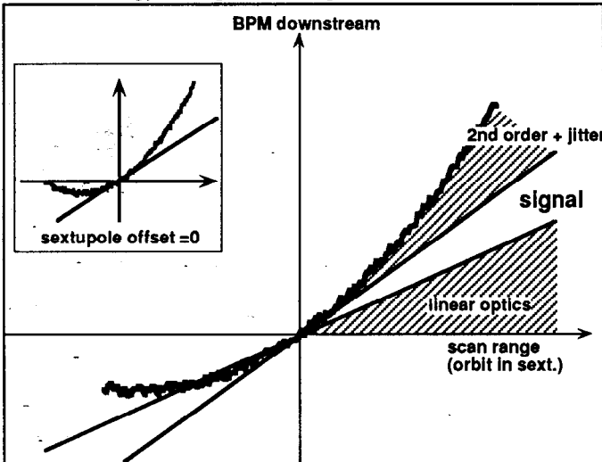
Figure 2. Sextupole offset effects reflected in orbit deflection versus orbit scan range. A beam is scanned about some predetermined reference line through a sextupole with an offset. The thick wiggly line shows the BPM reading downstream as a function of the incoming beam position or angle at a fixed point (or the strength of the corrector used for the scan). The same pattern with an aligned sextupole is shown in the box. When an offset is present, a very small linear signal and some additional wiggleness are added to this pattern which can be barely detectable.
