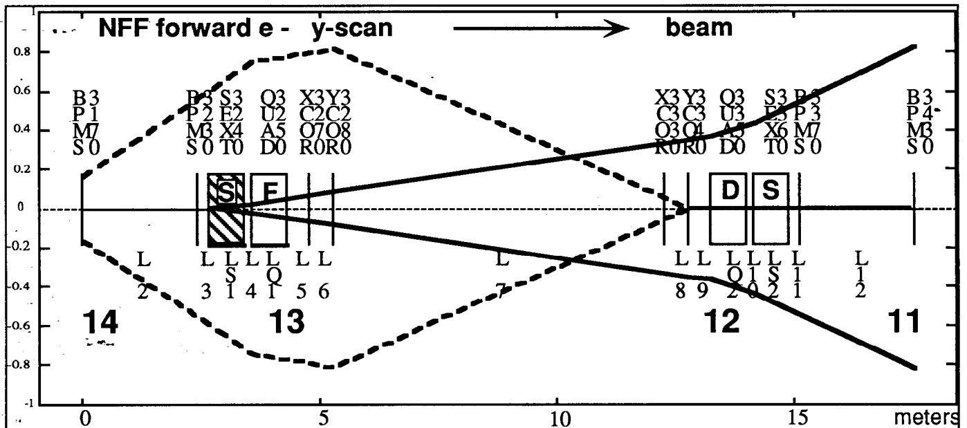
Figure 3. Optimized bump for sextupole offset measurement given realistic SLC CCS optics and hardware. The hatched block indicates the sextupole to be measured. The other blocks are focusing and defocusing quadrupoles and a powered-off sextupole. Vertical lines mark the locations of BPM's and corrector dipoles as indicated. The dashed lines are the bump envelopes in the exact shape. The solid lines are the propagation of the sextupole offset signals in the exact shape, although not to scale with the dashed lines.
