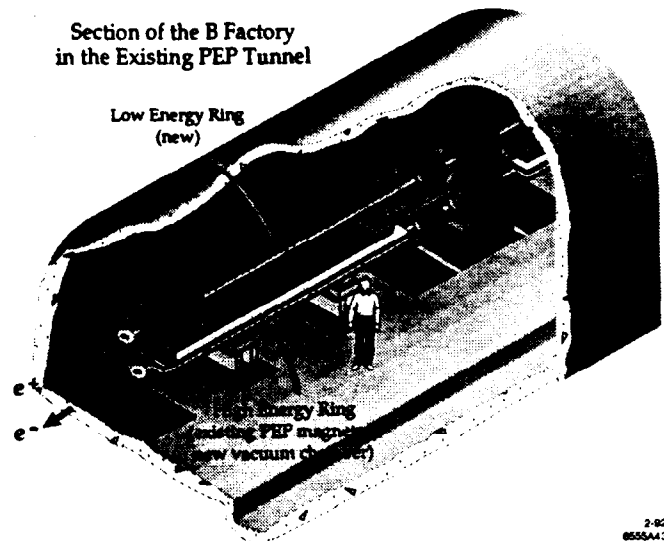
Fig. 1. Cutaway view of PEP-II tunnel.
