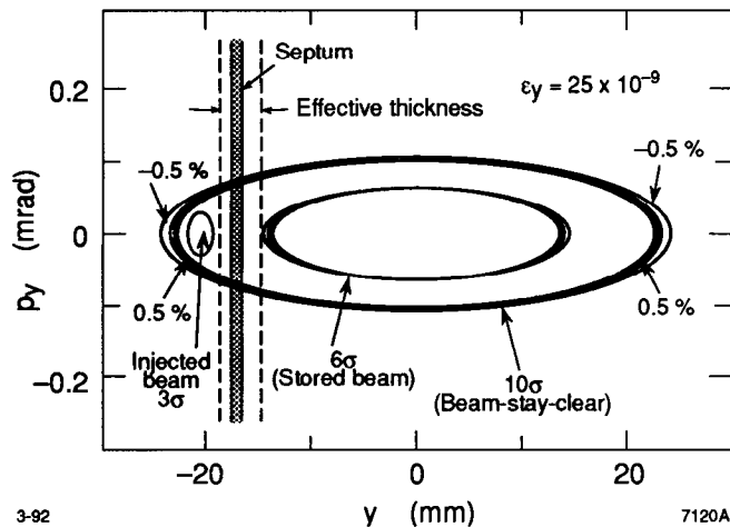
Fig. 4. Phase space diagram of injection acceptance for HER after chromatic correction.
