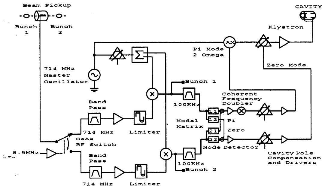
Figure 1. Block Diagram of the electronic feedback system. Two independent feedback loops control the barycentric mode (via the cavity RF phase) and the \pi mode (via an amplitude modulation of the cavity RF at 2\omega_\pi ).
