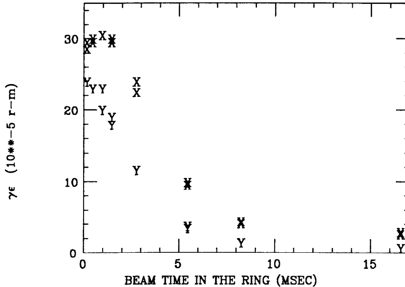
Measured extracted beam emittances versus storage time in the damping ring.
