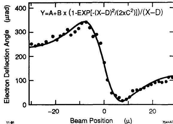
Figure 3. Beam-beam deflection fit at the interaction point.
