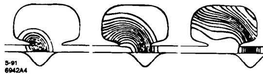
Fig. 6. The transient electromagnetic fields in a cavity as a bunch of electrons (shown in the position of the Gaussian curve below the axis) passes through the tube. The cavity in each view is the same cavity at a later instant.
