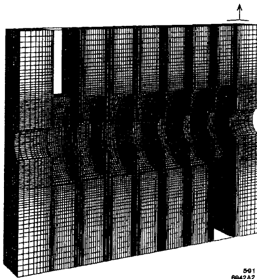
Fig. 4. Three-dimensional zoned model of the X-band structure shown in Fig. 1. About 500,000 zones are needed.
