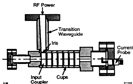
Fig. 3. Test structure for an X-band accelerator.
