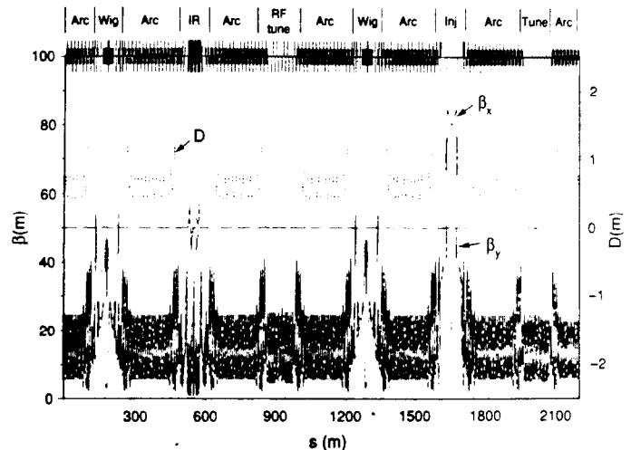
Fig. 3. Layout and optics functions for the LER. The lattice for the full ring is shown, starting and finishing at mid-arc in region 11.
