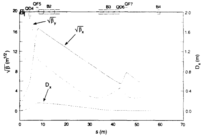
Fig. 7. Lattice functions for the first 60 m of the IR straight section of the HER. The B2 and B3 dipoles match the dispersion function to zero.
