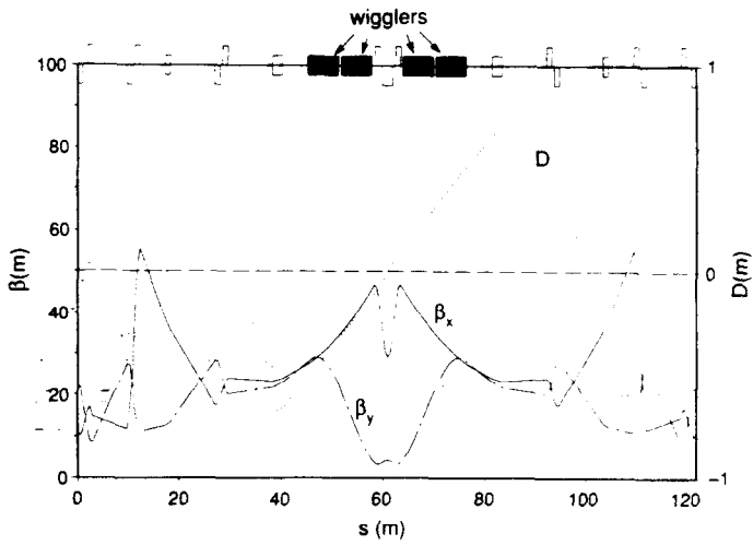
Fig. 4. Layout and optics functions for the wiggler straight sections of the LER. In conjunction with the dispersion function D , and its derivative, the wigglers increase the emittance of the low-energy beam. In addition, the wigglers can decrease the damping time of the low-energy beam so that it is equal to that of the high-energy beam.
