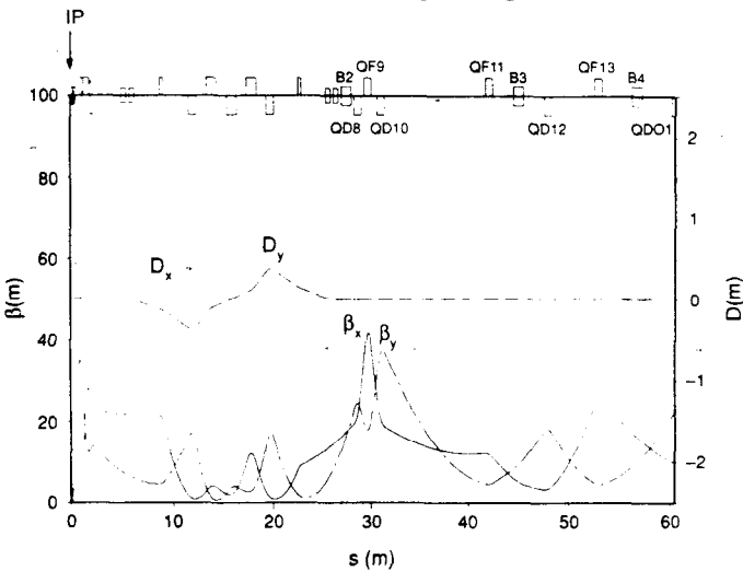
Fig. 5. Layout and optics functions for the right-hand half of the IR straight section of the LER. The quadrupoles QD8 through QF13 match the beta functions into the dispersion suppressor.
