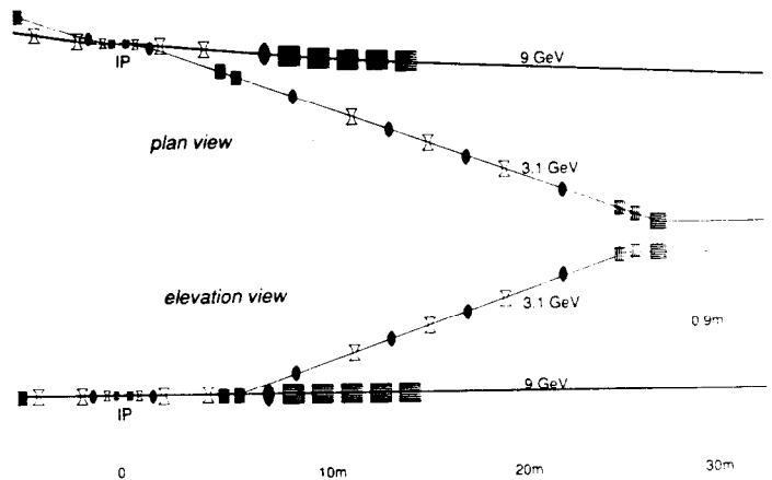
Fig. 2. Magnetic separation of the high and low energy beams. The initial horizontal separation is accomplished by a combination of a permanent magnet dipole followed by three offset permanent magnet quadrupoles. Separation is achieved by exploiting the energy difference between the beams. Once the beams are separated a system of vertically bending dipoles elevates the LER above the HER.
