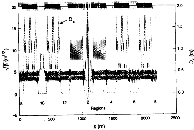
Fig. 6. Lattice functions \sqrt{\beta_x} , \sqrt{\beta_y} , and D_x (horizontal dispersion function) for the complete HER, starting at region 8. The collision region (region 2) is shown in the center of the figure.
