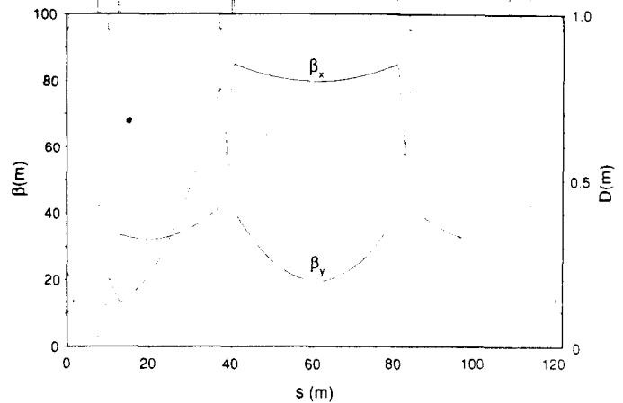
Fig. 8. Layout and optics functions for the injection straight section of the LER. The injection point is at the center of the figure, in the middle of the long straight section. Beta functions in this region are easily adjustable to match injection requirements.
