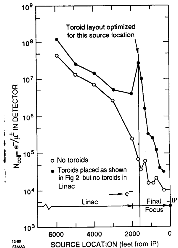
Fig. 3. Number of electrons impinging on a collimator which yield one muon in the detector ( N_{coll} ) as a function of source location in the linac and final focus.
