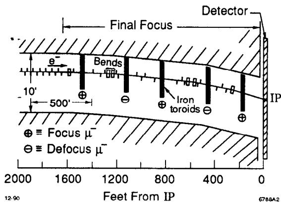
Fig. 2. Schematic of the final focus beam line used for this study. Note the different scale in the transverse and longitudinal directions.
