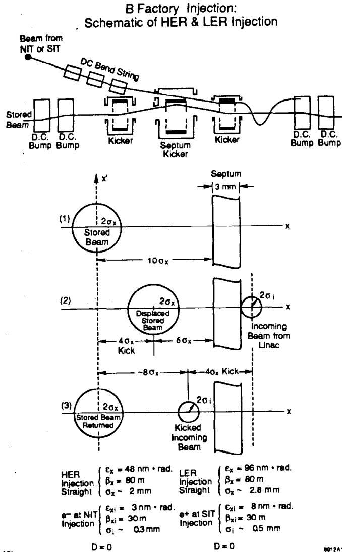
Fig. 3 Schematic of Injection Kicker System, and horizontal transverse phase space ( x, x' ) of stored and incoming beams during three successive steps of the injection process (HER and LER). The diameters of the stored and incoming beams are not drawn to scale.
