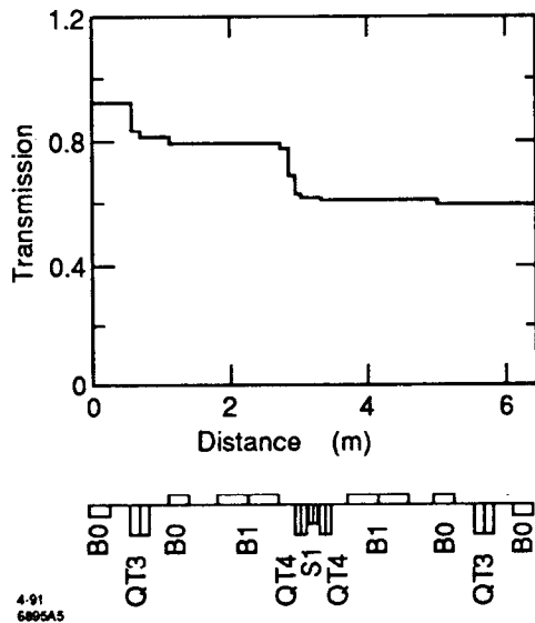
Figure 5. Simulated transmission through the East Turn.
