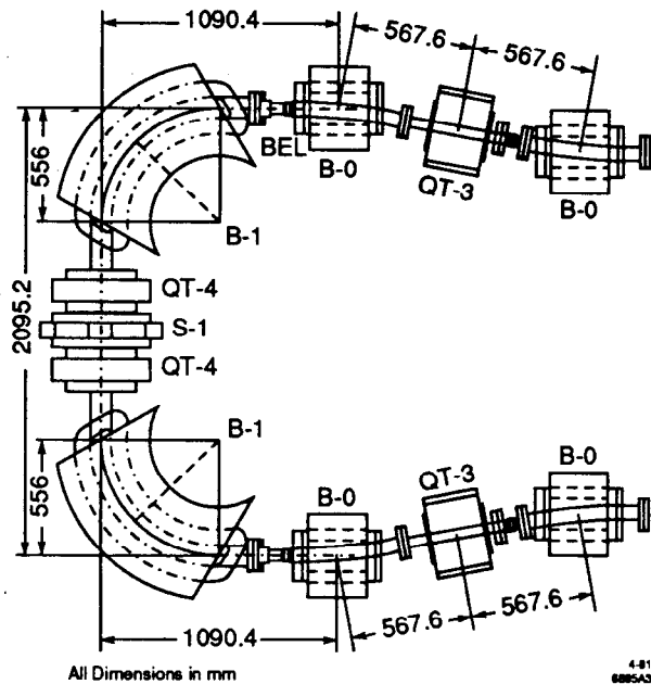
Figure 2. Mechanical layout.
