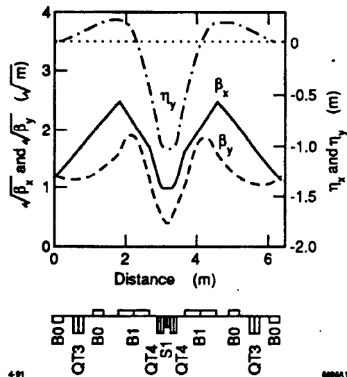
Figure 1. Optical functions of the 180° Turns.
