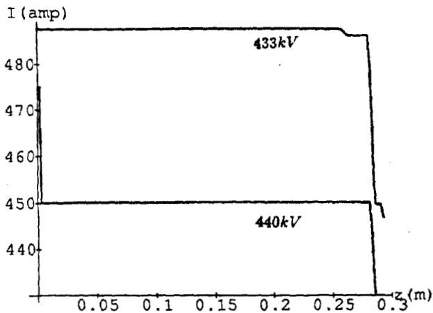
Figure 4 DC current as a function of z
