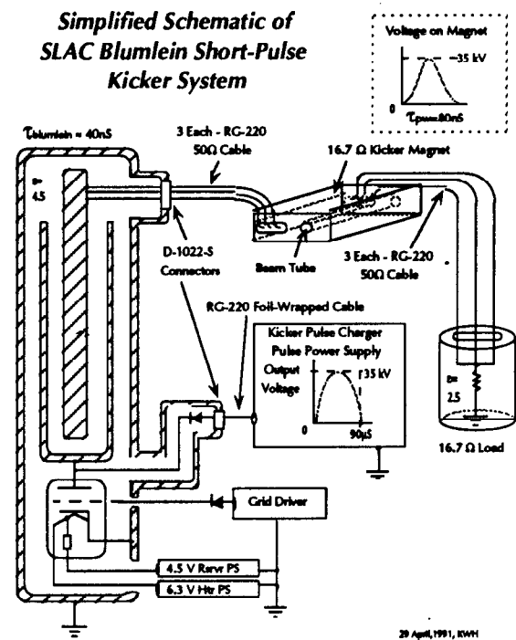
Figure 1. Short-Pulse Blumlein Kicker System.
