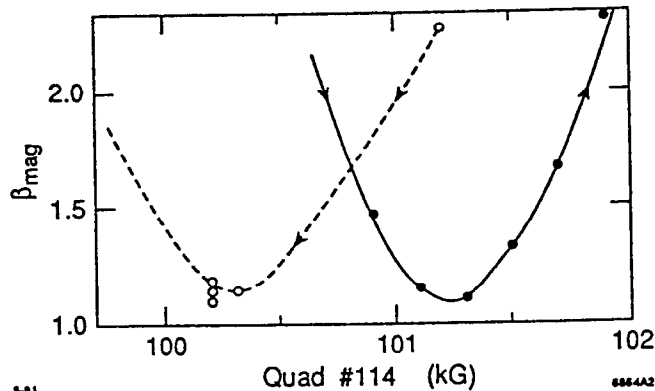
Figure 2: Betatron Match Sensitivity.
