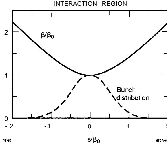
Figure 6: The longitudinal bunch distribution overlaid on a graph of the beta-junction in the vicinity of the IR. In the case depicted, many particles lie in the wings of the beam waist.
