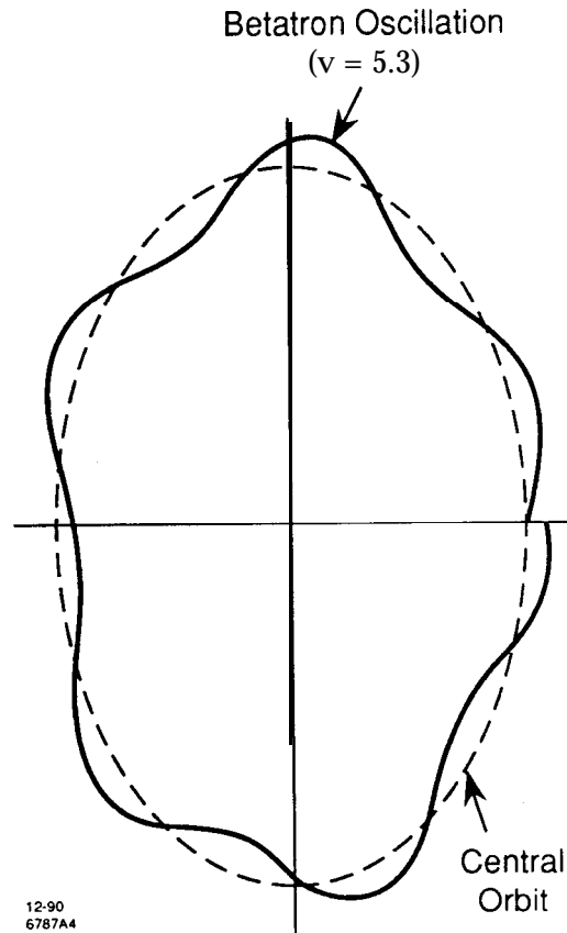
Figure 4: A betatron oscillation.
