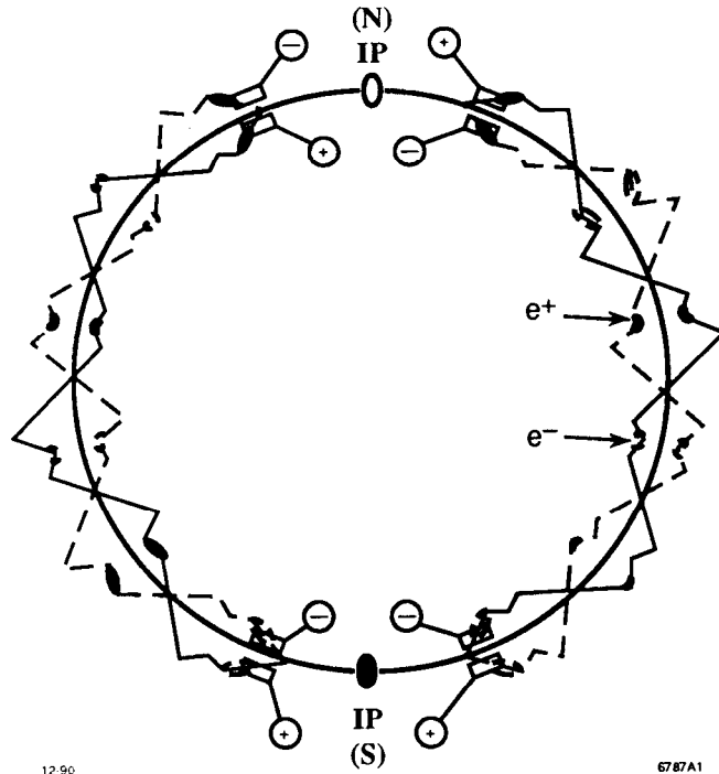
Figure 1: A schematic depiction of the “pretzel orbits” in the CESR storage ring. The circle represents the central orbit; the other solid line is the positron orbit; and the dashed line is the electron orbit. The electron and positron bunches avoid each other, because they are deflected onto different orbits by the electric fields situated on either side of the interaction region.
