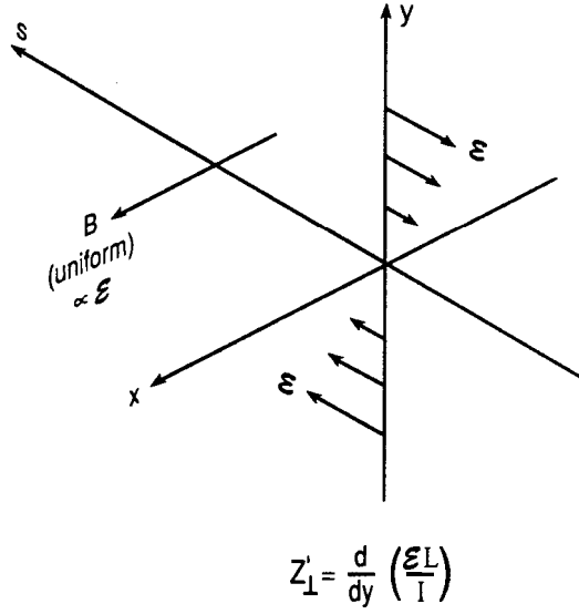
Figure 8: Fields of a mode that drives the transverse mode-coupling instability. Near the axis, the magnetic field is transverse and nearly constant and the electric field is longitudinal and linearly dependent on a transverse coordinate.
