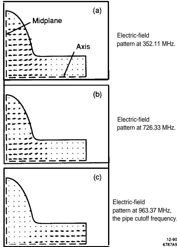
Figure 9: One quadrant of an rf cavity with only two trapped modes. The mode at 352 MHz is the accelerating mode. The mode at 963 MHz propagates down the pipe. Only the mode at 726 MHz remains to create unwanted parasitic impedance.
