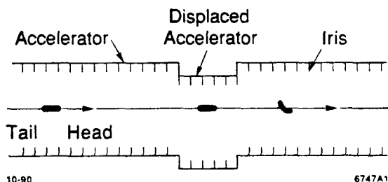
Fig. 1 Displaced accelerator structures produce wakefields effects.
