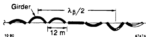
Fig. 3 Use of distorted accelerator girders to make structure offsets at the betatron spatial frequency.
