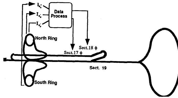
Fig. 2 The feedforward loop to stabilize the scavenger beam energy.
