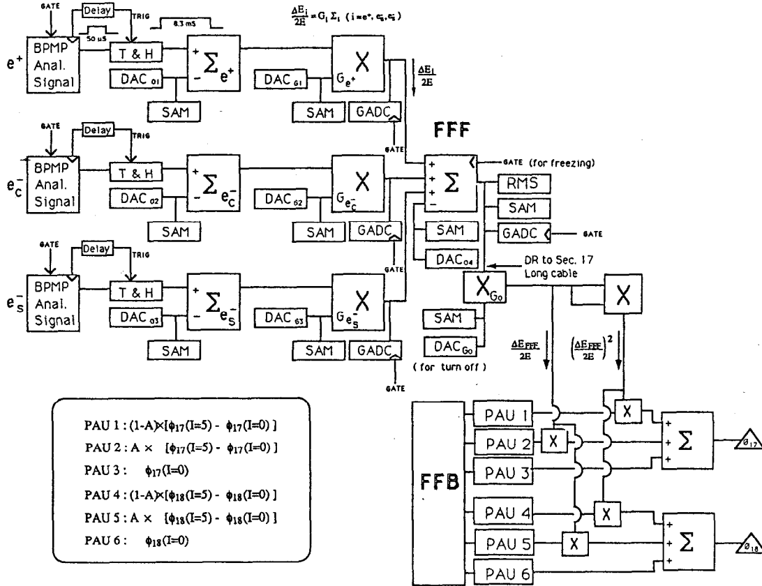
Fig. 3 The block diagram showing the overall loop structure.
