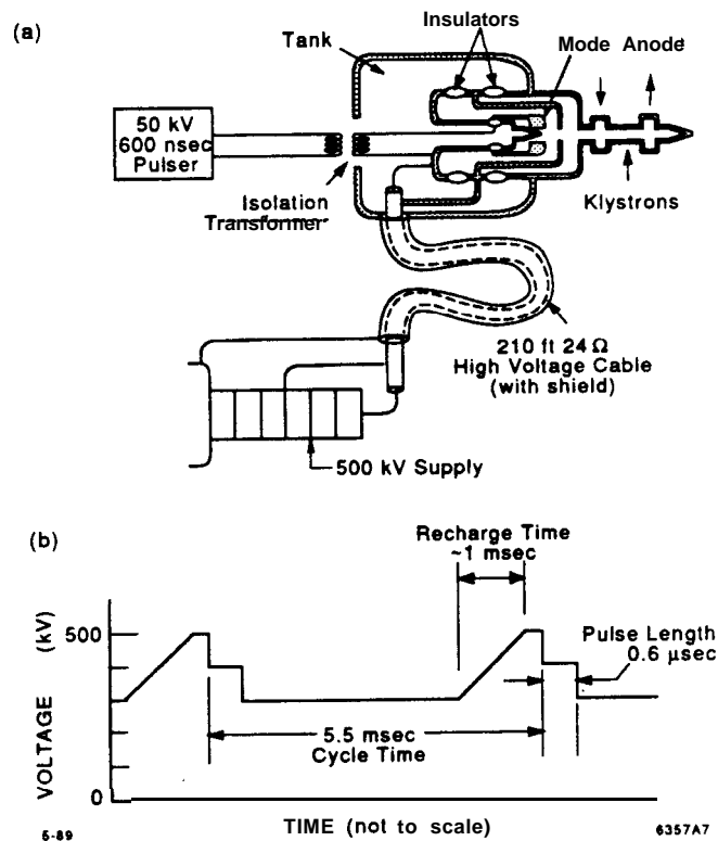
FIGURE 6 Electrical system: (a) Circuit diagram. (b) Klystron voltage vs. time.
